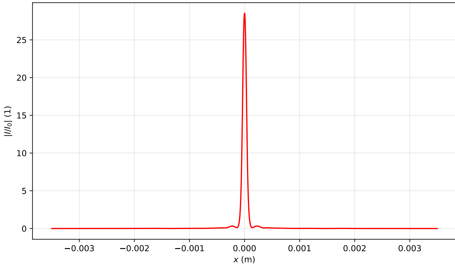
Intensity profile I(x, y = 0, z = 2.388)/I_0 , P_{in}=3.5P_{cr} , artificial time
